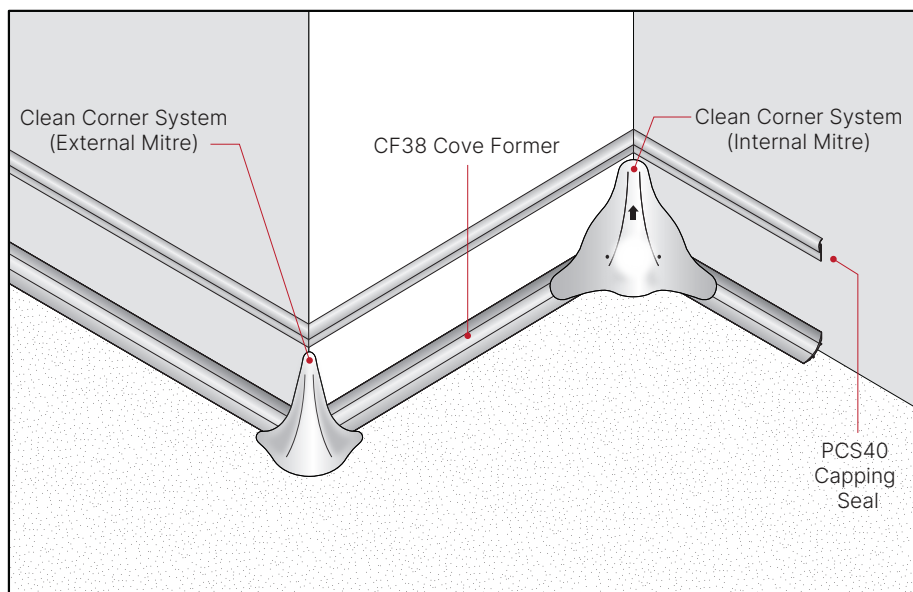
Gerflor Clean Corner System internal and external mitres with Gradus CF38 Cove Former and PCS40 Capping Seal
